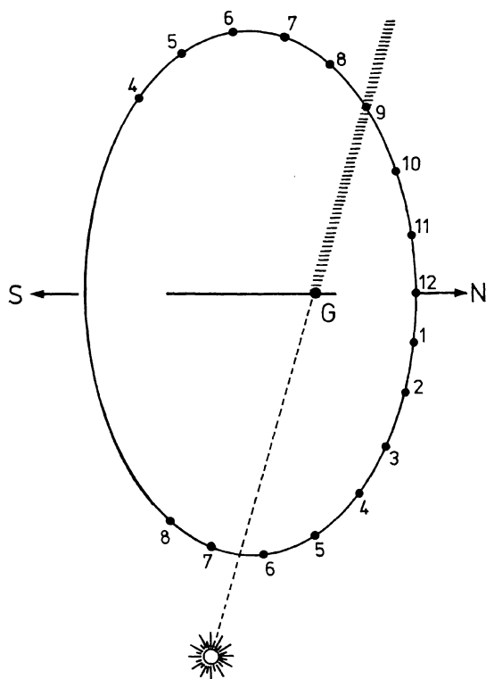
Figure 1. View from above of the prototype of an equator projection sundial. G is a vertical gnomon at a point on the line of dates. The shadow of the gnomon indicates the true solar time on the circumference of the ellipse (here 9 o'clock, May 1).
